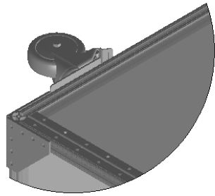
DETAIL B Casters for Easier Transportation
