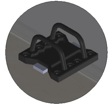
DETAIL C Locking Bar Mechanism to Ensure that Trapdoors Remain Closed
