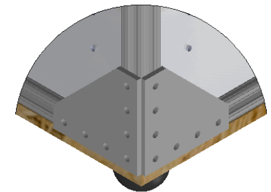
DETAIL E Aluminum 8020 Strut and Right Angle Brackets for Increased Stability
